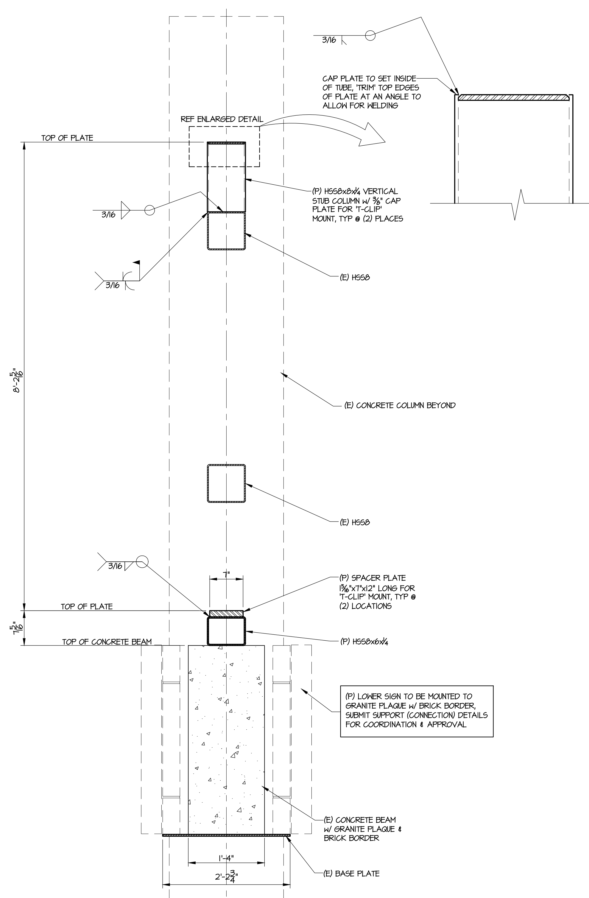
2 8-1 SECTION THRU PROPOSED SIGN AND SUPPORT 1'-1'-0"
