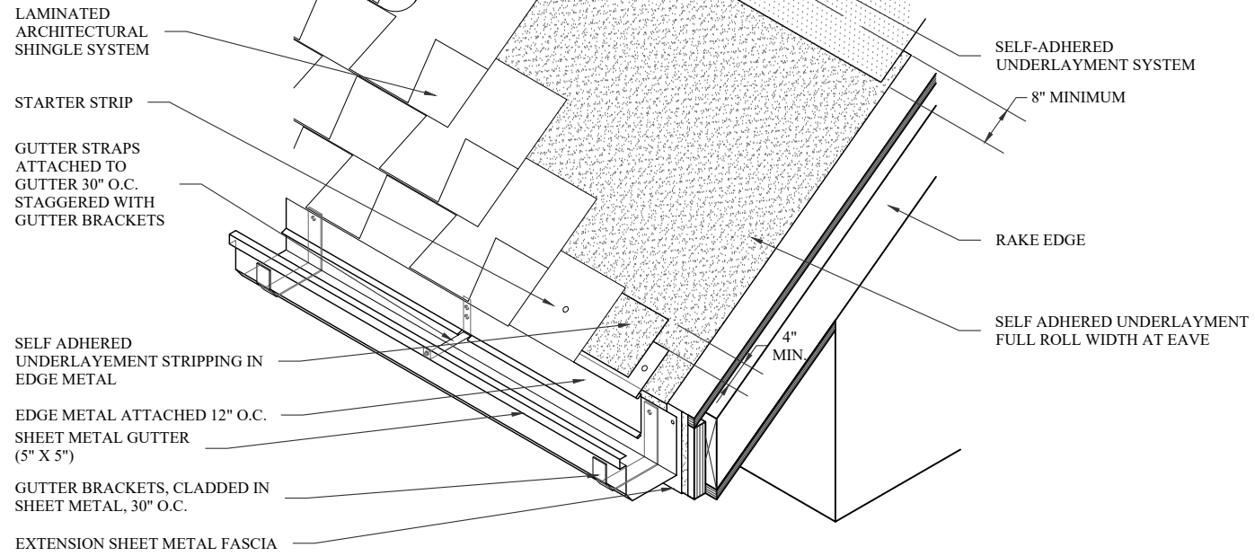
ROOF EDGE WITH GUTTER DETAIL 6/D-1.2
