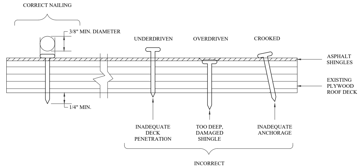
SHINGLE FASTENING STANDARD DETAIL 2/D-1.1
